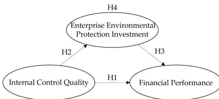
Figure 1. Theoretical model.
